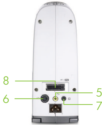
Inputs (rear view shown)
